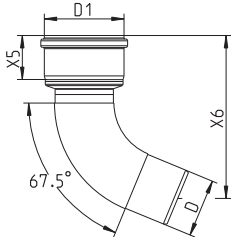
TOILET ADAPTOR 68° TYPE 858.090
