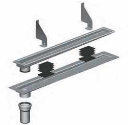
Series 37X for tiled floor with liquid membrane
