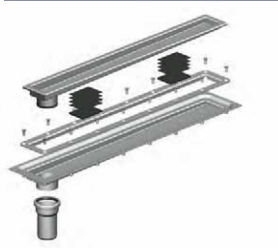
Series 395 for tiled floor with sheet membrane
